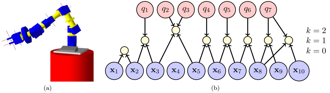
Fig. 11: Experiment with a simulated 7-DOF-manipulator consisting of 10 body parts. Body part \mathbf{x}_4 was occluded and, thus, never observed. (a) Picture of the simulated robot. (b) After 10 training samples, the Bayesian network has converged to the correct kinematic structure.
