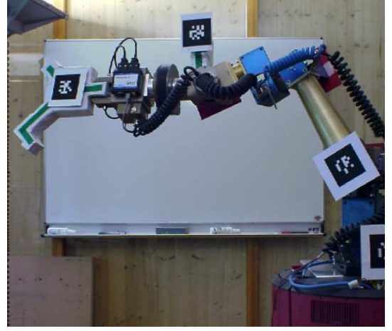
(b) 7-DOF robot
